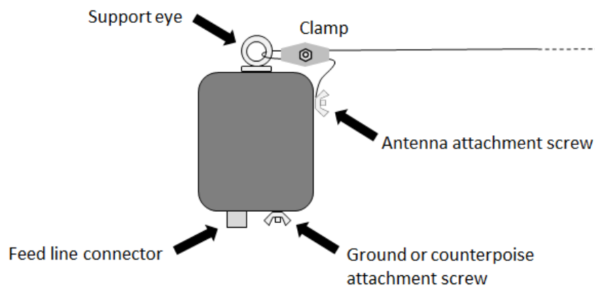
EFHW Transformer
