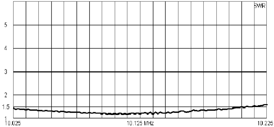
TYPICAL VSWR PLOT
