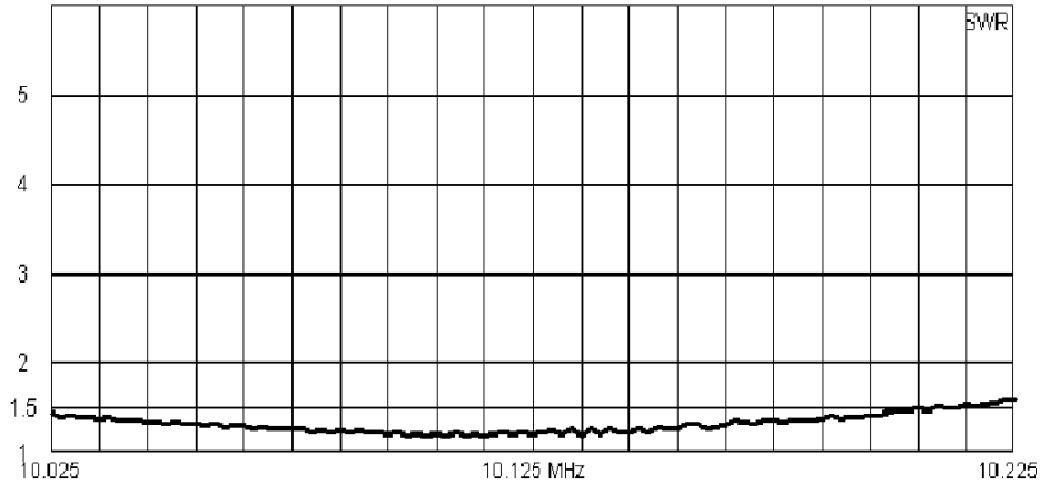
TYPICAL VSWR PLOT
